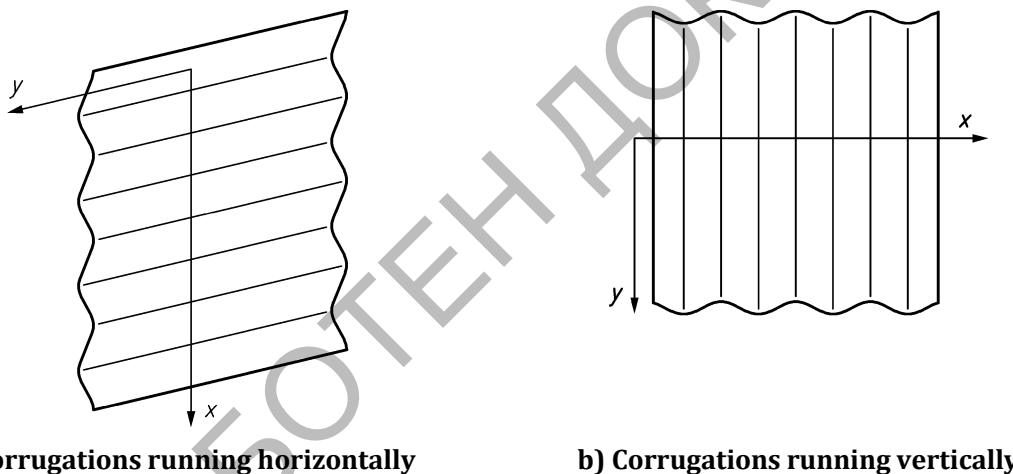
Figure 4.3 — Corrugated sheeting and silo wall orientations
