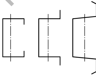
Figure 5.5 a) — Cold-formed stiffeners with edge stiffened flanges EN 1993-1-3 identifiers: buckling curve b
