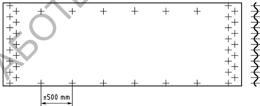
Figure 5.4 — Typical bolt arrangement for a panel of a corrugated silo
