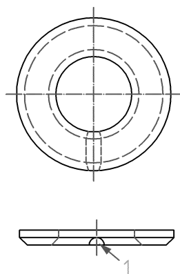
Figure J.4 — Preparation of the washer for use under the nut
