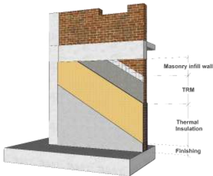
Figure 7. Combined seismic and energy retrofitting with TRM and thermal insulation (Pohoryles et al., 2020)
