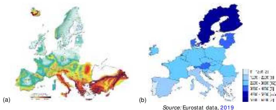
Figure 2. (a) European seismic hazard map (Giardini et al., 2014) and (b) European climatic zones map in terms of HDD
